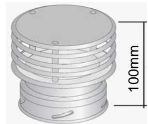
Flue Cowl. Part no. 7162
